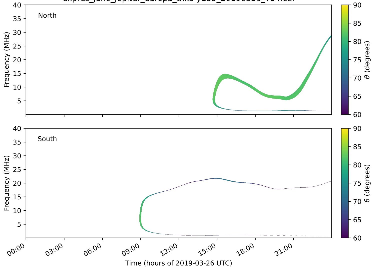
expres_juno_jupiter_europa_txka-y235_20190326_v14.cdf
