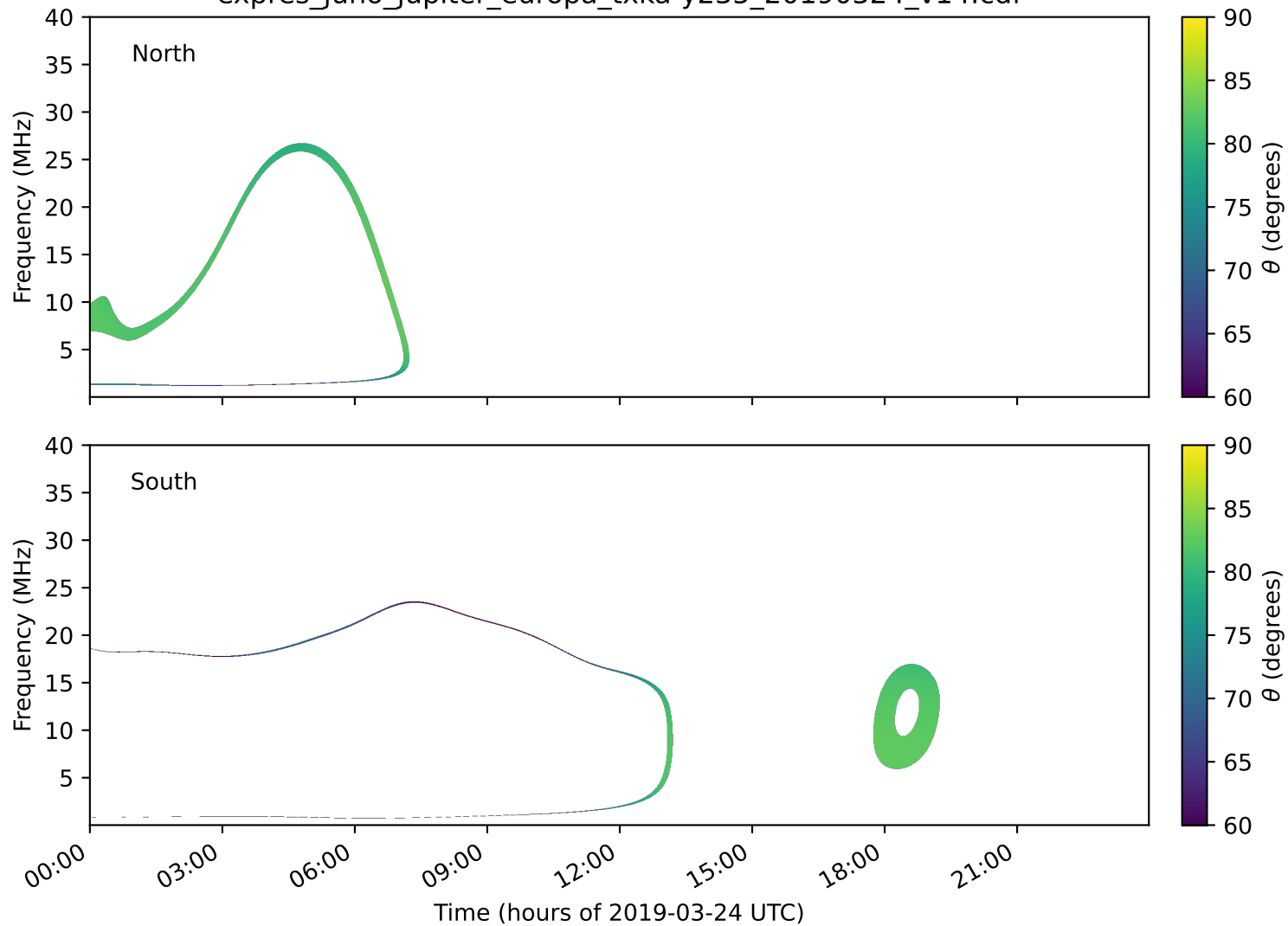
expres_juno_jupiter_europa_txka-y235_20190324_v14.cdf
