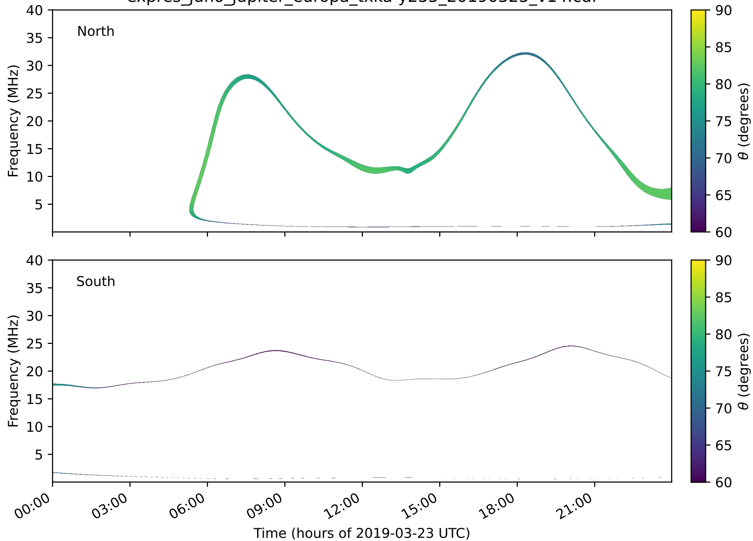
expres_juno_jupiter_europa_txka-y235_20190323_v14.cdf
