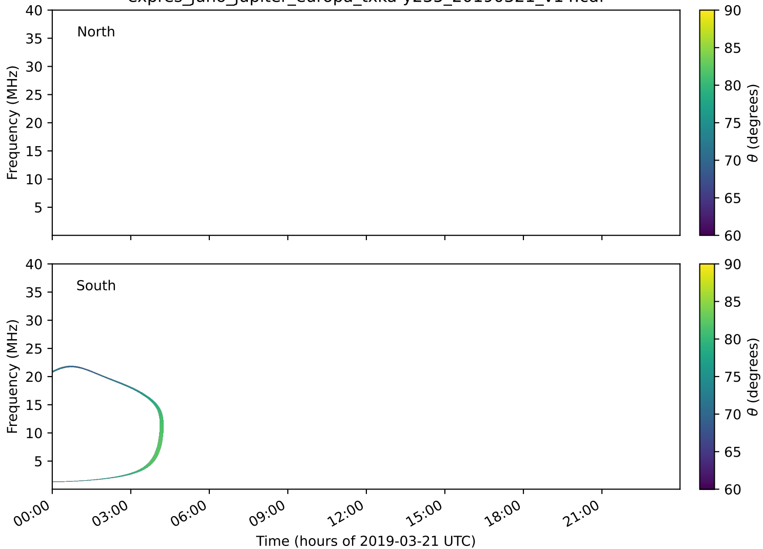
expres_juno_jupiter_europa_txka-y235_20190321_v14.cdf
