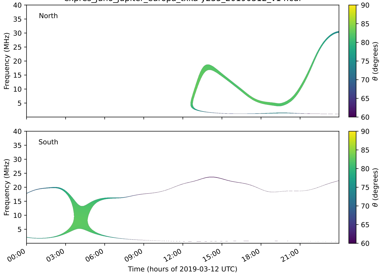
expres_juno_jupiter_europa_txka-y235_20190312_v14.cdf
