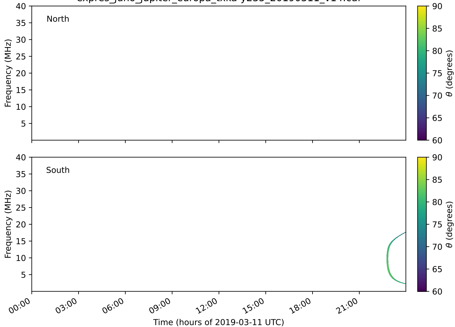
expres_juno_jupiter_europa_txka-y235_20190311_v14.cdf
