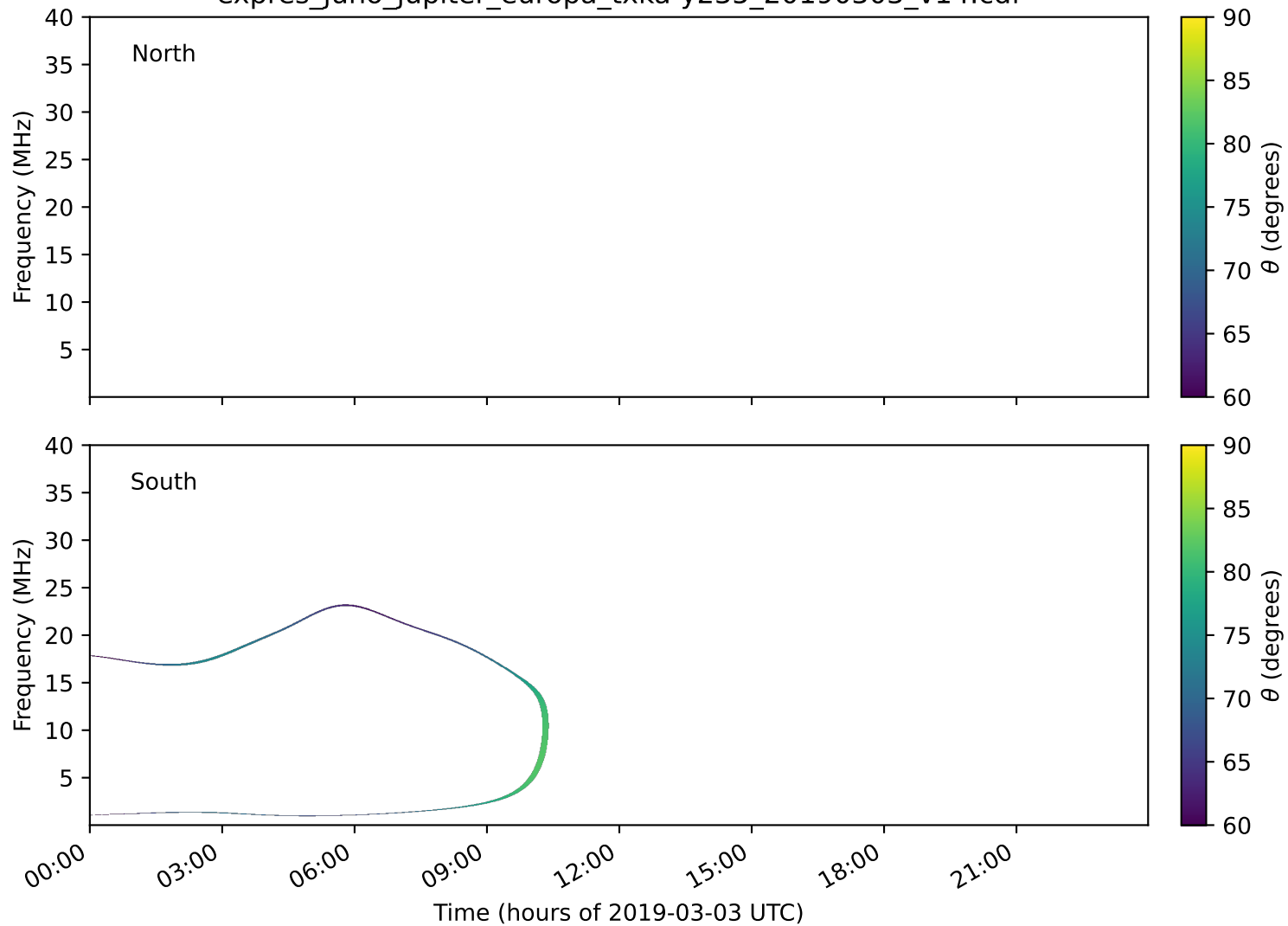
expres_juno_jupiter_europa_txka-y235_20190303_v14.cdf
