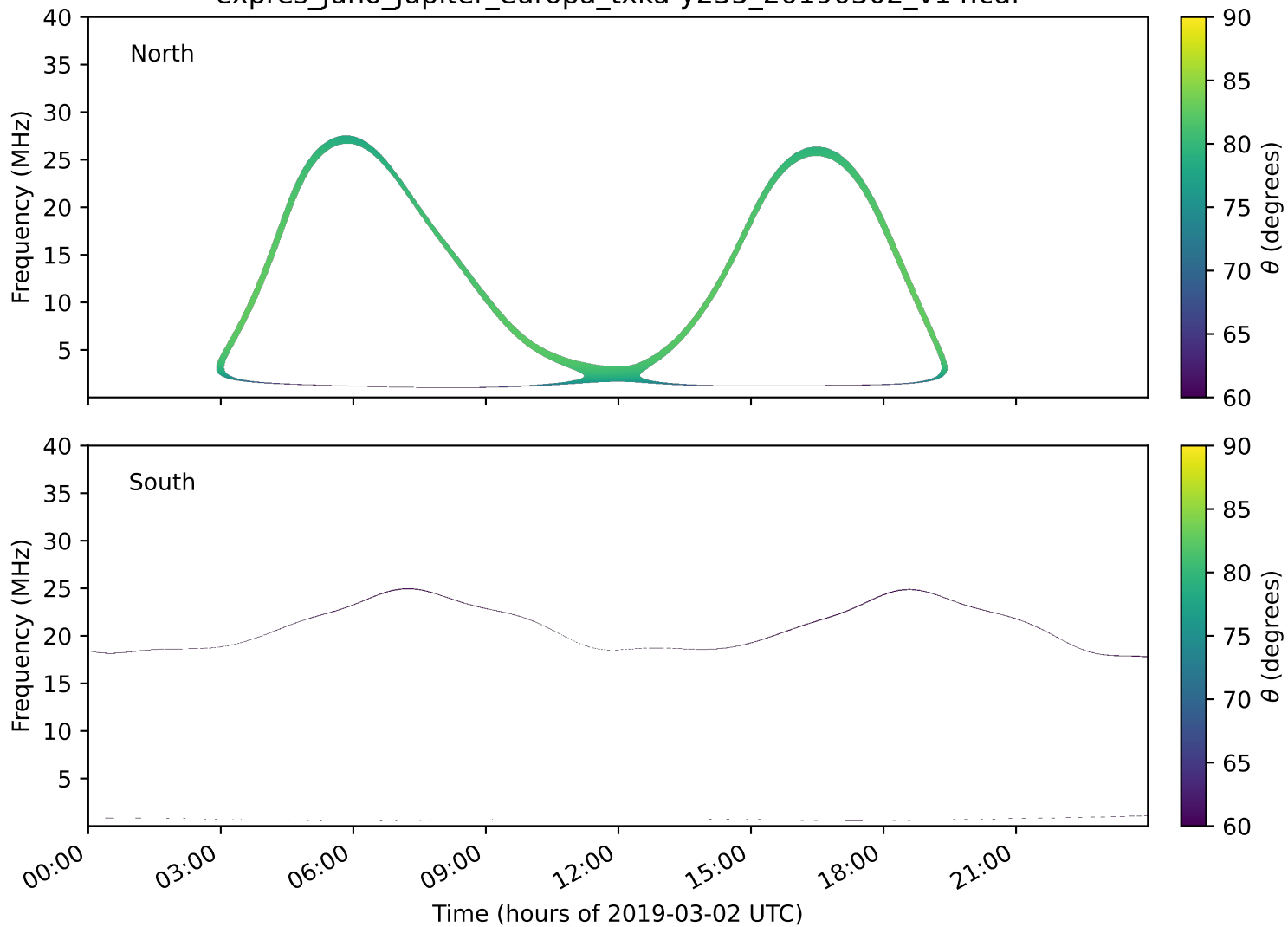
expres_juno_jupiter_europa_txka-y235_20190302_v14.cdf
