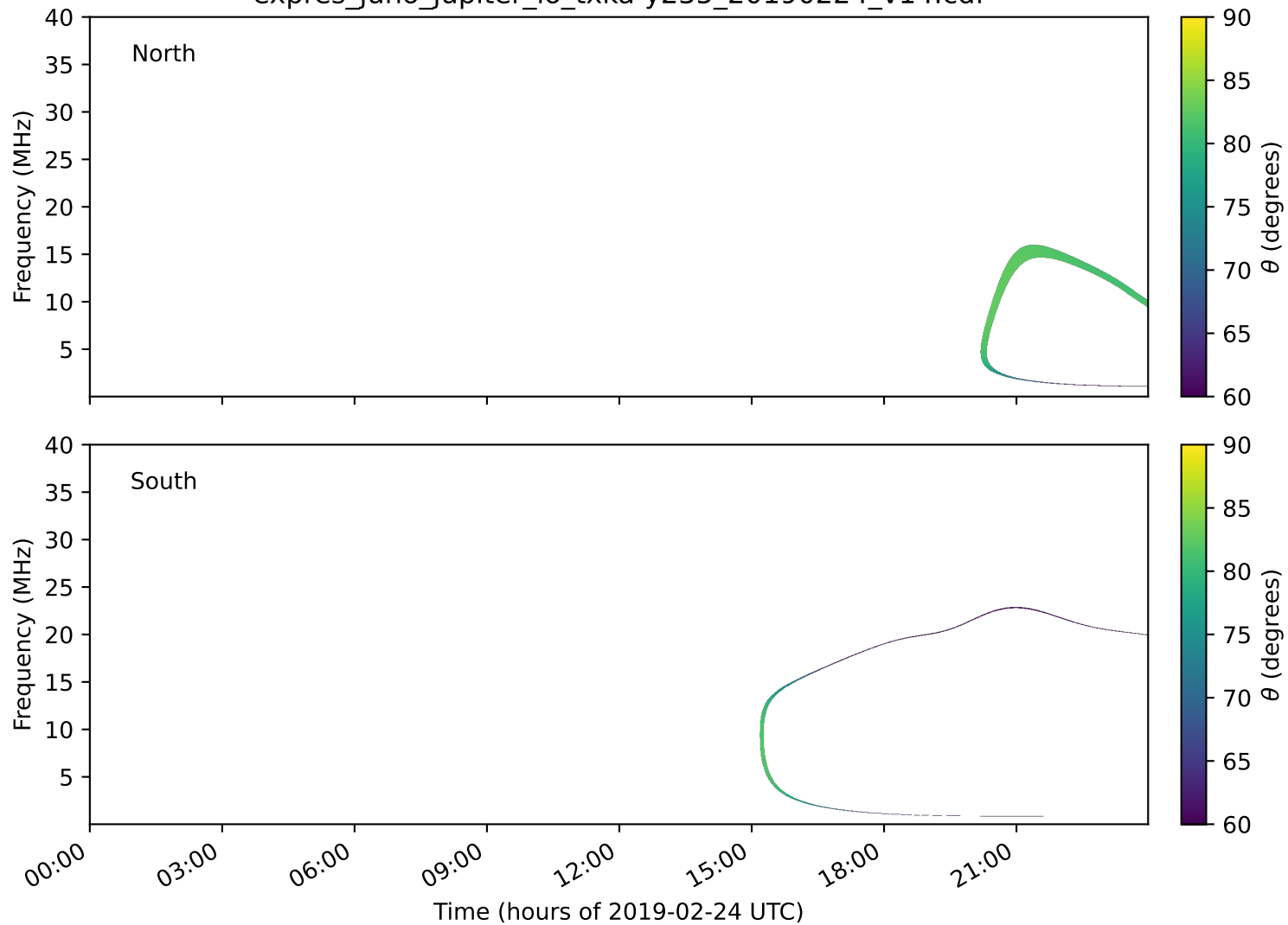
expres_juno_jupiter_io_txka-y235_20190224_v14.cdf
