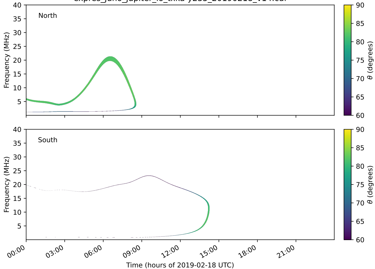
expres_juno_jupiter_io_txka-y235_20190218_v14.cdf
