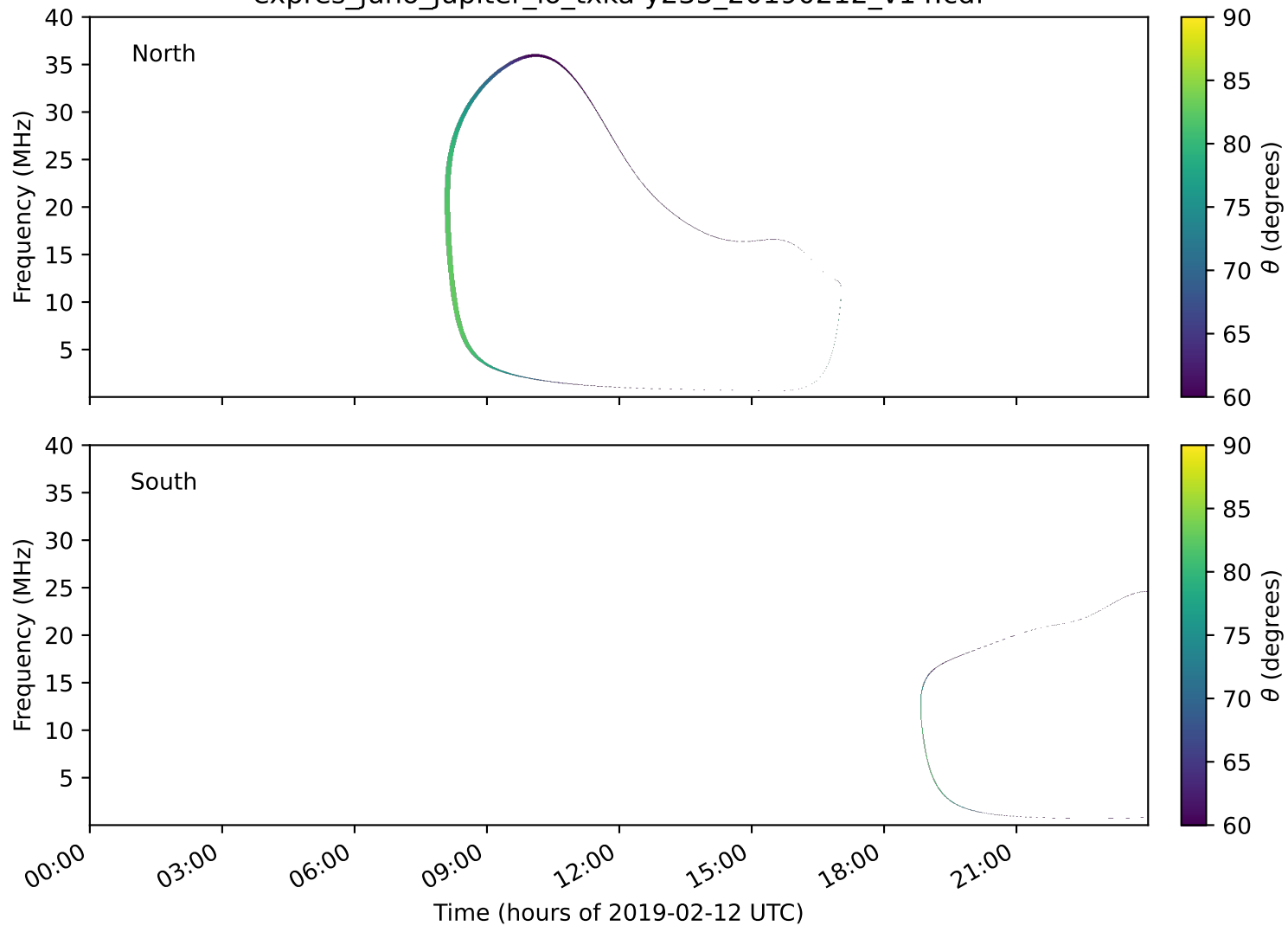
expres_juno_jupiter_io_txka-y235_20190212_v14.cdf
