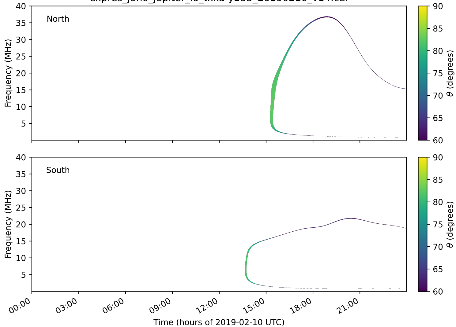
expres_juno_jupiter_io_txka-y235_20190210_v14.cdf
