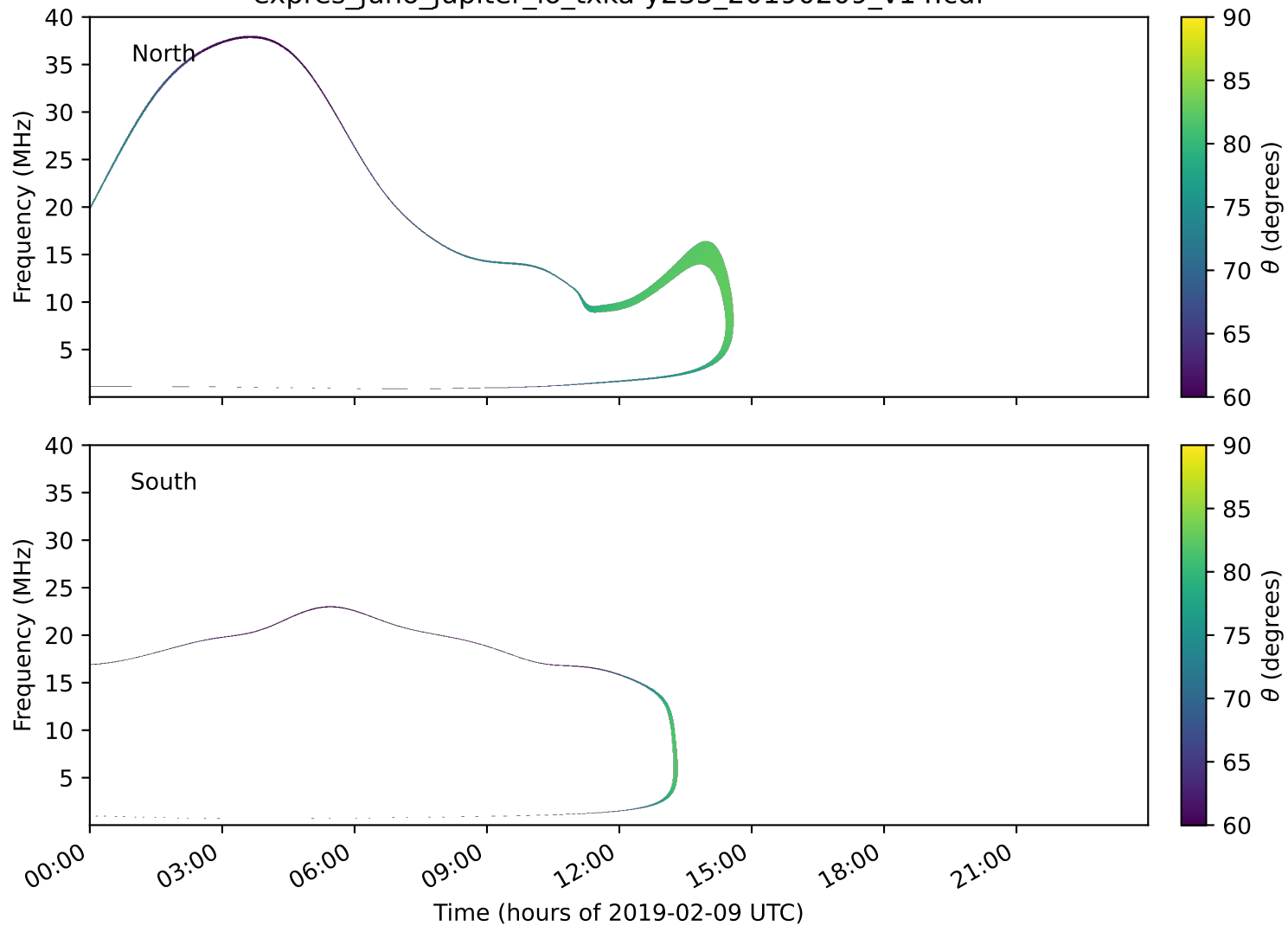
expres_juno_jupiter_io_txka-y235_20190209_v14.cdf
