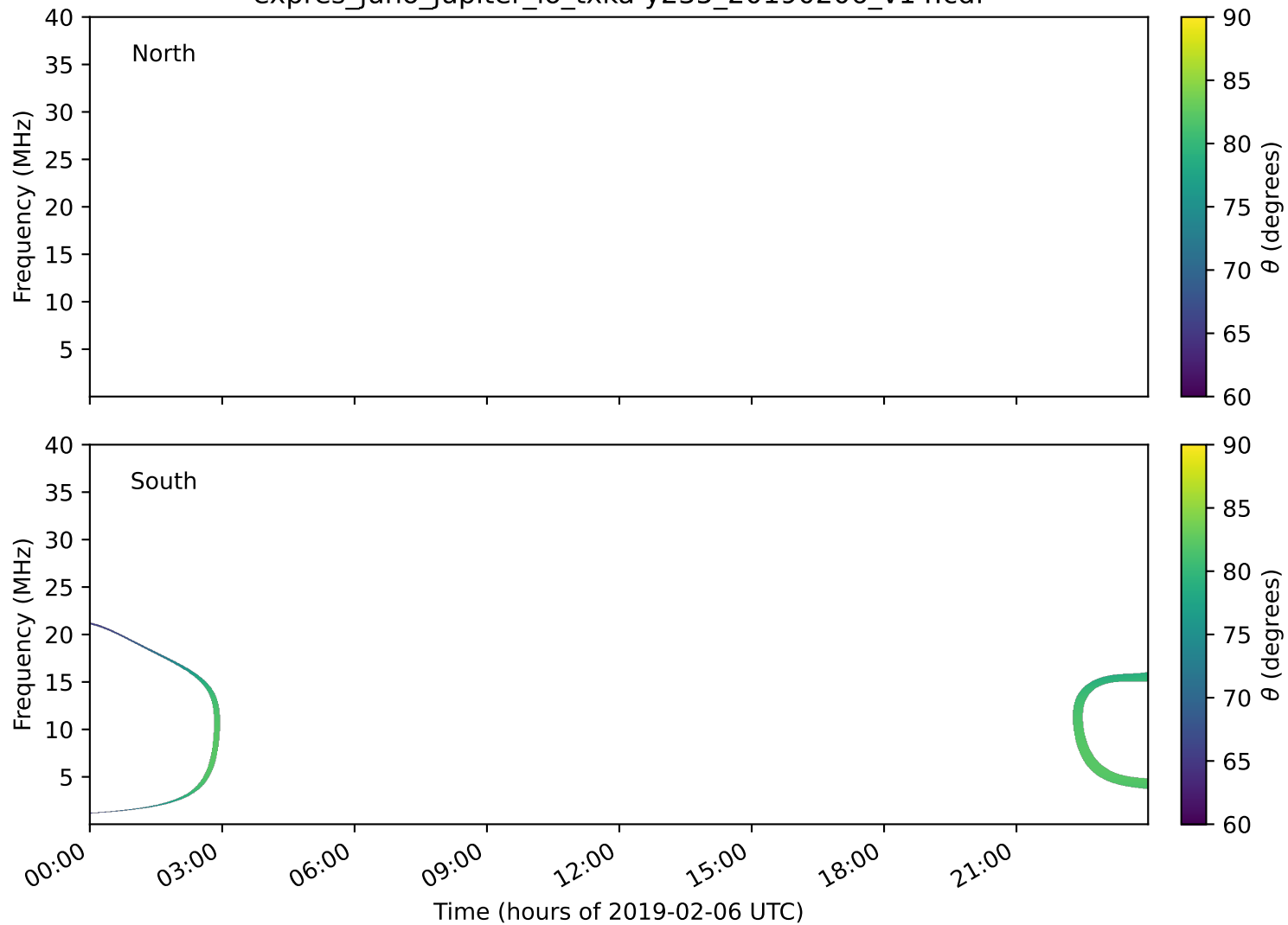
expres_juno_jupiter_io_txka-y235_20190206_v14.cdf
