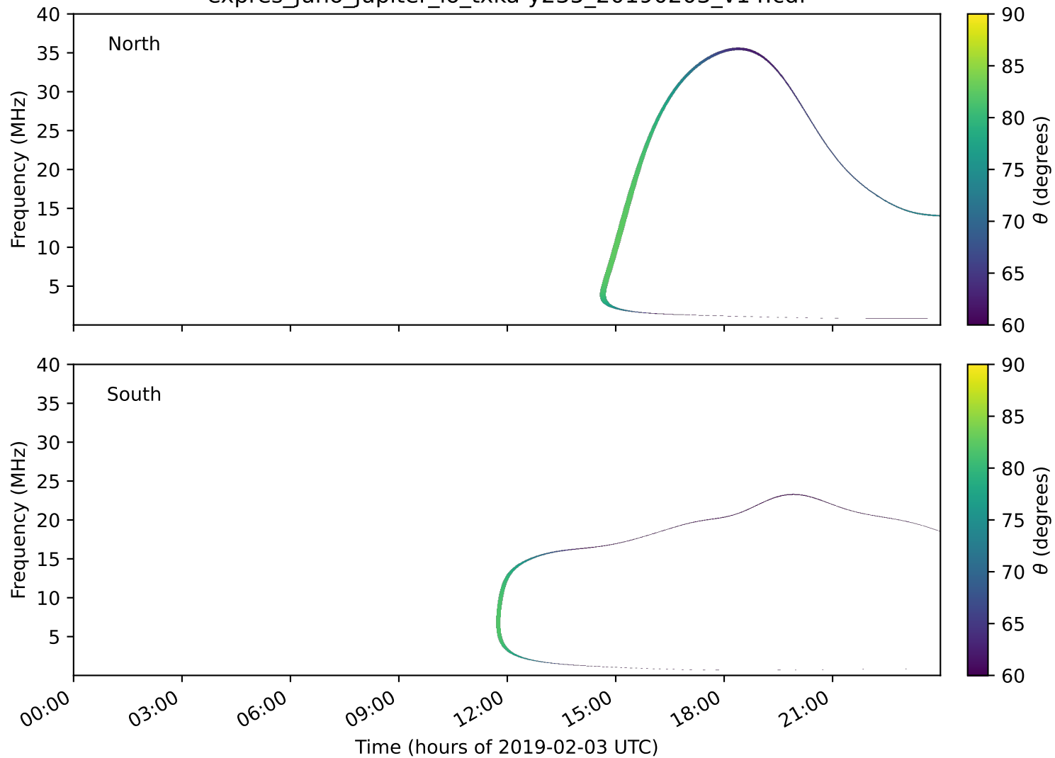
expres_juno_jupiter_io_txka-y235_20190203_v14.cdf
