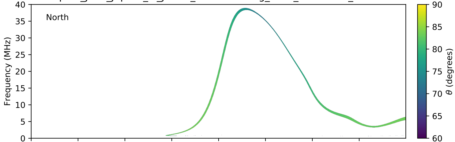
expres_juno_jupiter_io_jrm09_lossc-wid1deg_3kev_20190228_v01.cdf
