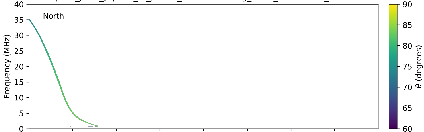
expres_juno_jupiter_io_jrm09_lossc-wid1deg_3kev_20190227_v01.cdf
