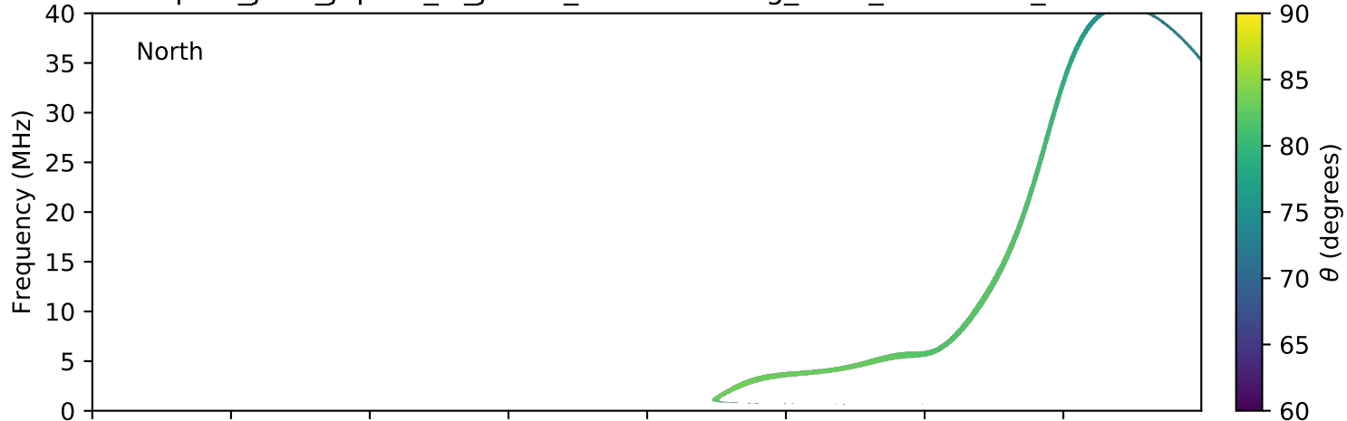
expres_juno_jupiter_io_jrm09_lossc-wid1deg_3kev_20190226_v01.cdf
