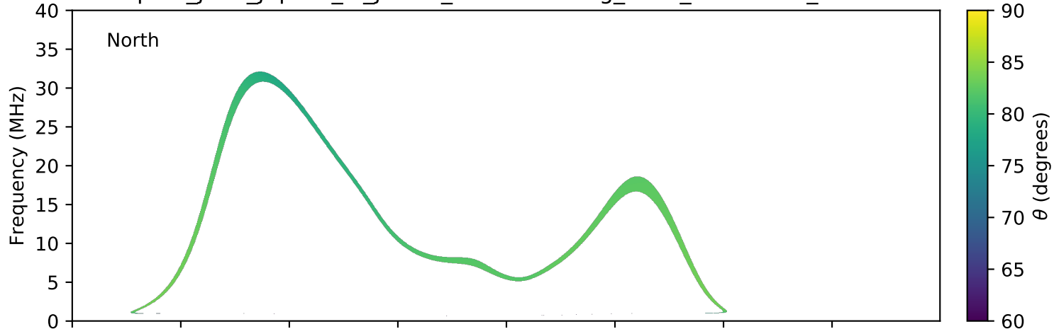
expres_juno_jupiter_io_jrm09_lossc-wid1deg_3kev_20190223_v01.cdf
