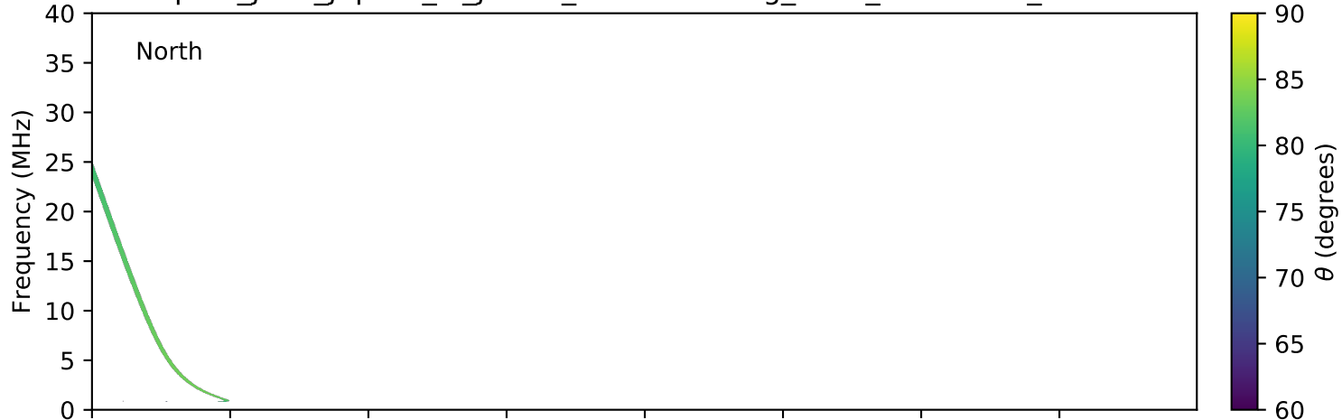
expres_juno_jupiter_io_jrm09_lossc-wid1deg_3kev_20190220_v01.cdf
