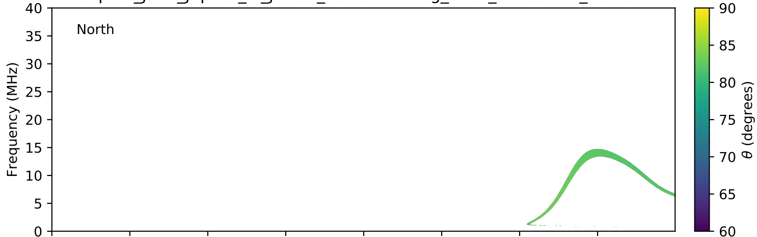
expres_juno_jupiter_io_jrm09_lossc-wid1deg_3kev_20190217_v01.cdf
