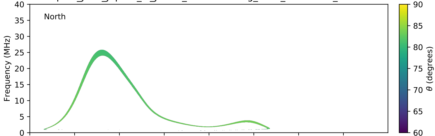
expres_juno_jupiter_io_jrm09_lossc-wid1deg_3kev_20190216_v01.cdf
