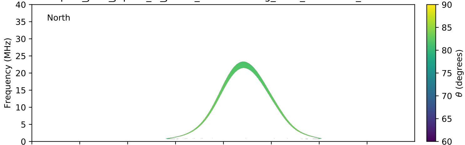
expres_juno_jupiter_io_jrm09_lossc-wid1deg_3kev_20190214_v01.cdf
