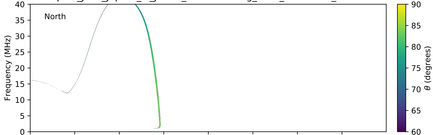
expres_juno_jupiter_io_jrm09_lossc-wid1deg_3kev_20190211_v01.cdf
