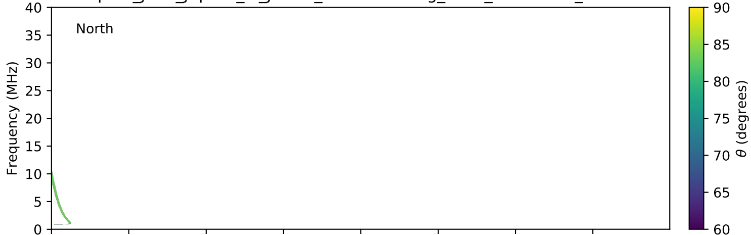
expres_juno_jupiter_io_jrm09_lossc-wid1deg_3kev_20190206_v01.cdf
