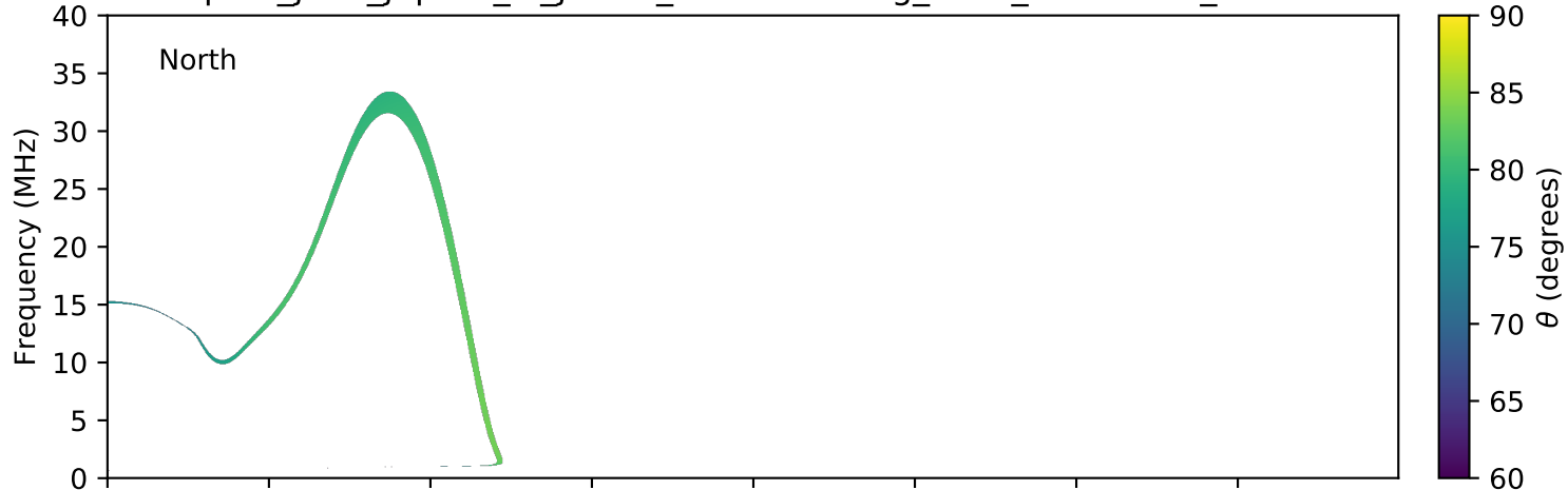
expres_juno_jupiter_io_jrm09_lossc-wid1deg_3kev_20190204_v01.cdf
