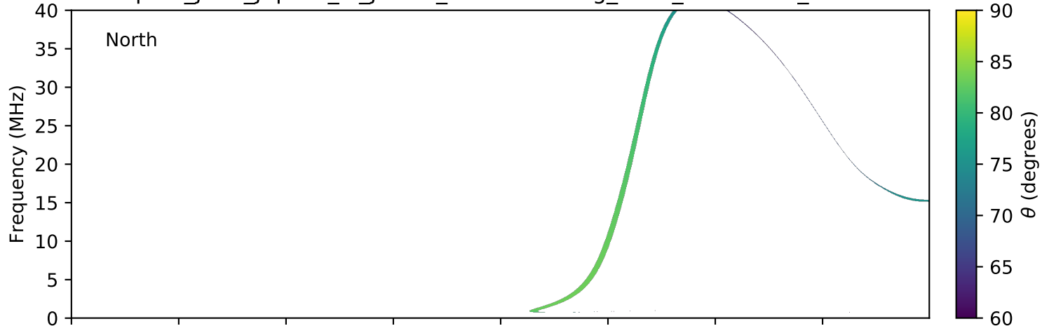
expres_juno_jupiter_io_jrm09_lossc-wid1deg_3kev_20190203_v01.cdf
