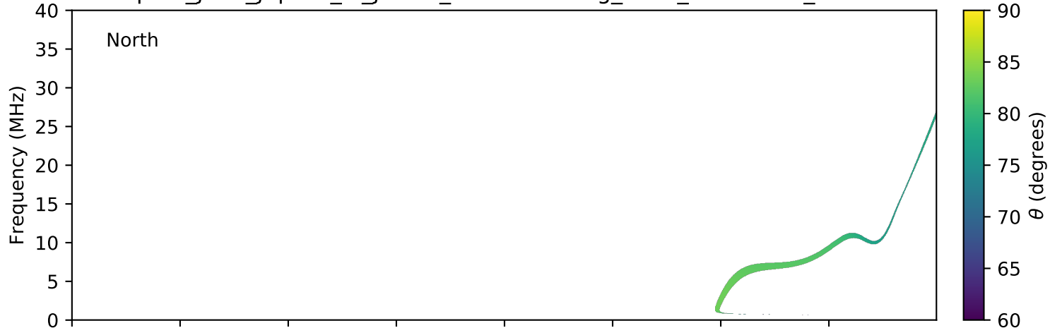
expres_juno_jupiter_io_jrm09_lossc-wid1deg_3kev_20190201_v01.cdf
