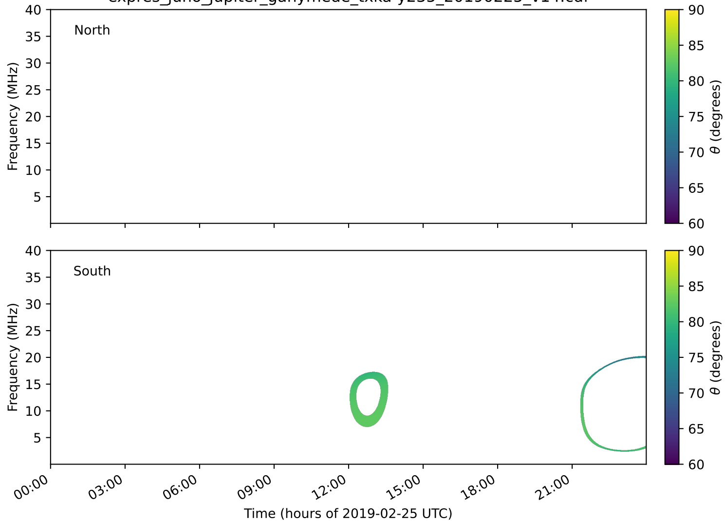
expres_juno_jupiter_ganymede_txka-y235_20190225_v14.cdf
