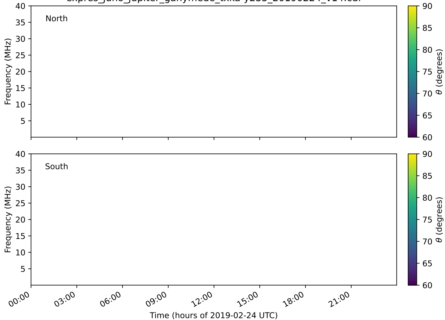
expres_juno_jupiter_ganymede_txka-y235_20190224_v14.cdf
