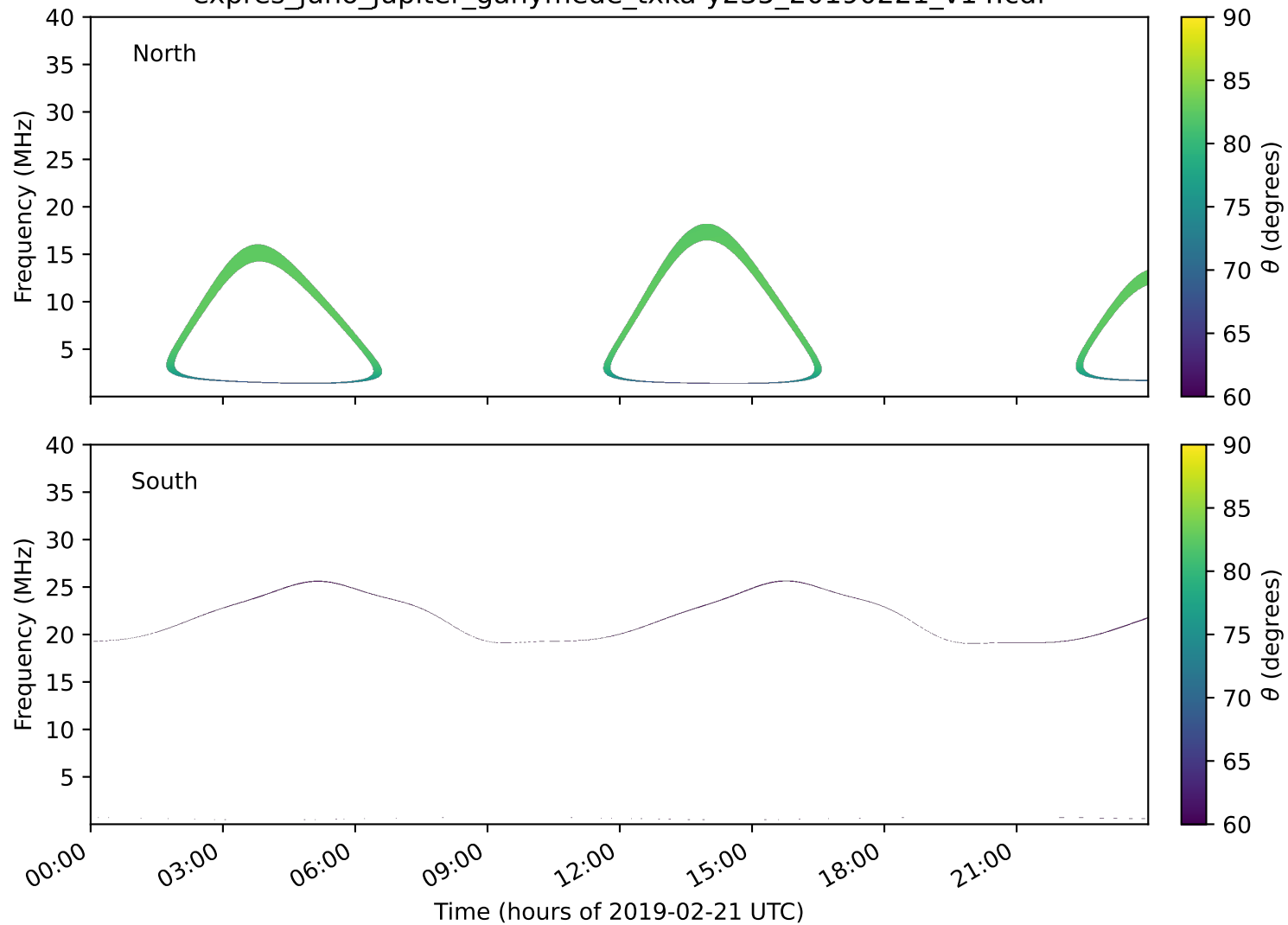
expres_juno_jupiter_ganymede_txka-y235_20190221_v14.cdf
