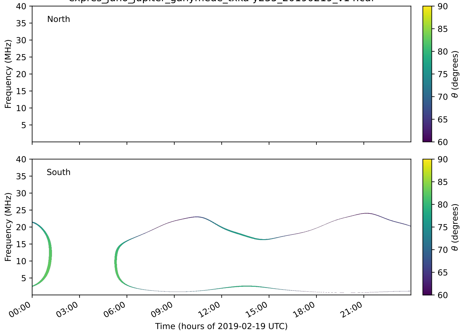
expres_juno_jupiter_ganymede_txka-y235_20190219_v14.cdf
