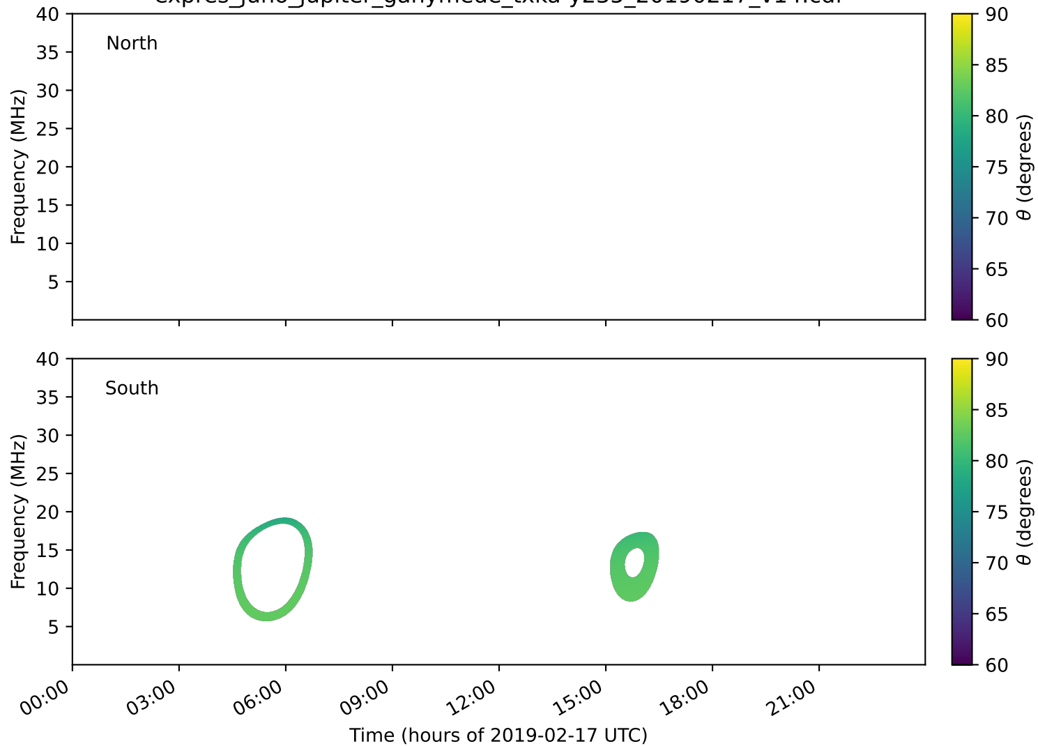
expres_juno_jupiter_ganymede_txka-y235_20190217_v14.cdf
