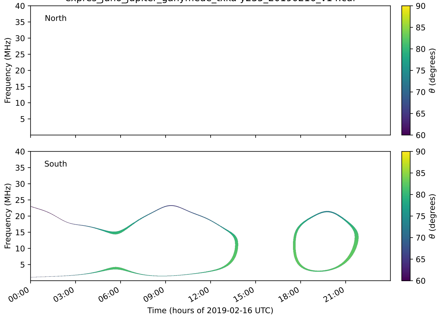
expres_juno_jupiter_ganymede_txka-y235_20190216_v14.cdf
