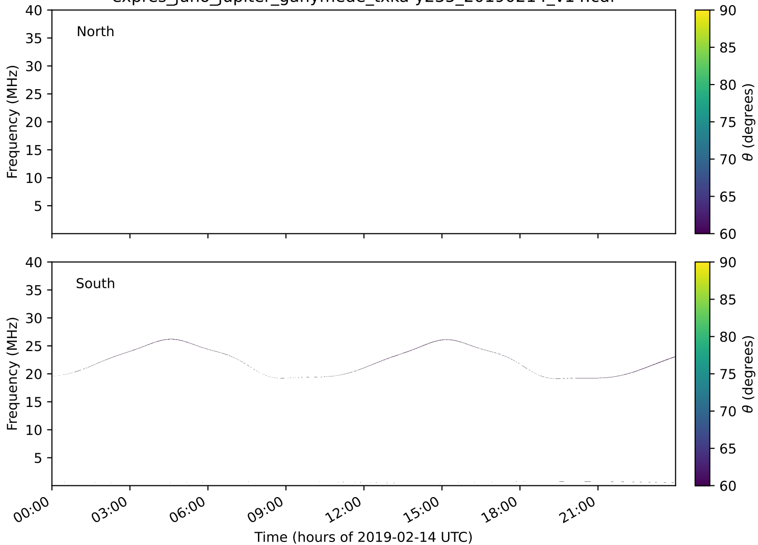
expres_juno_jupiter_ganymede_txka-y235_20190214_v14.cdf
