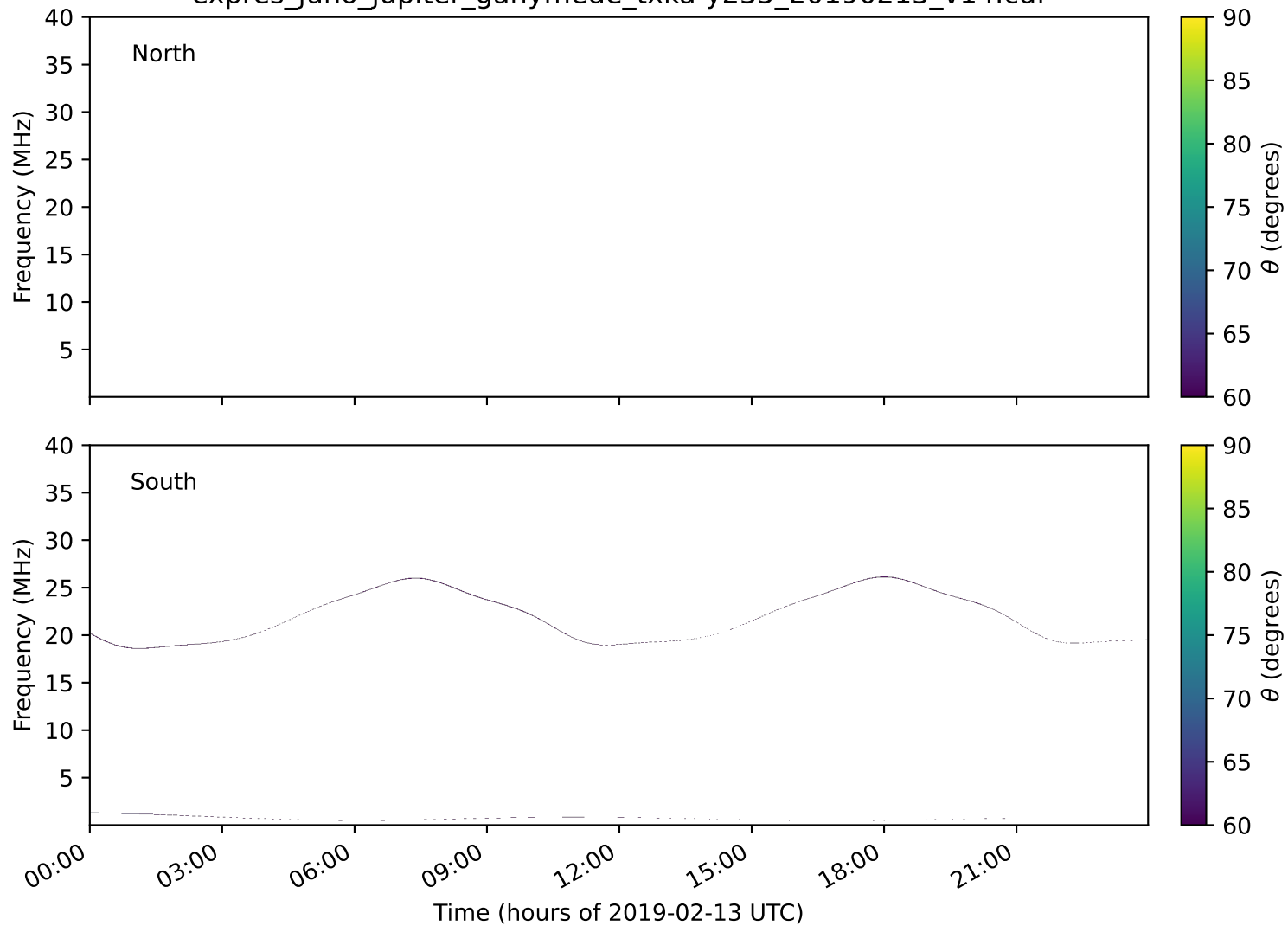
expres_juno_jupiter_ganymede_txka-y235_20190213_v14.cdf
