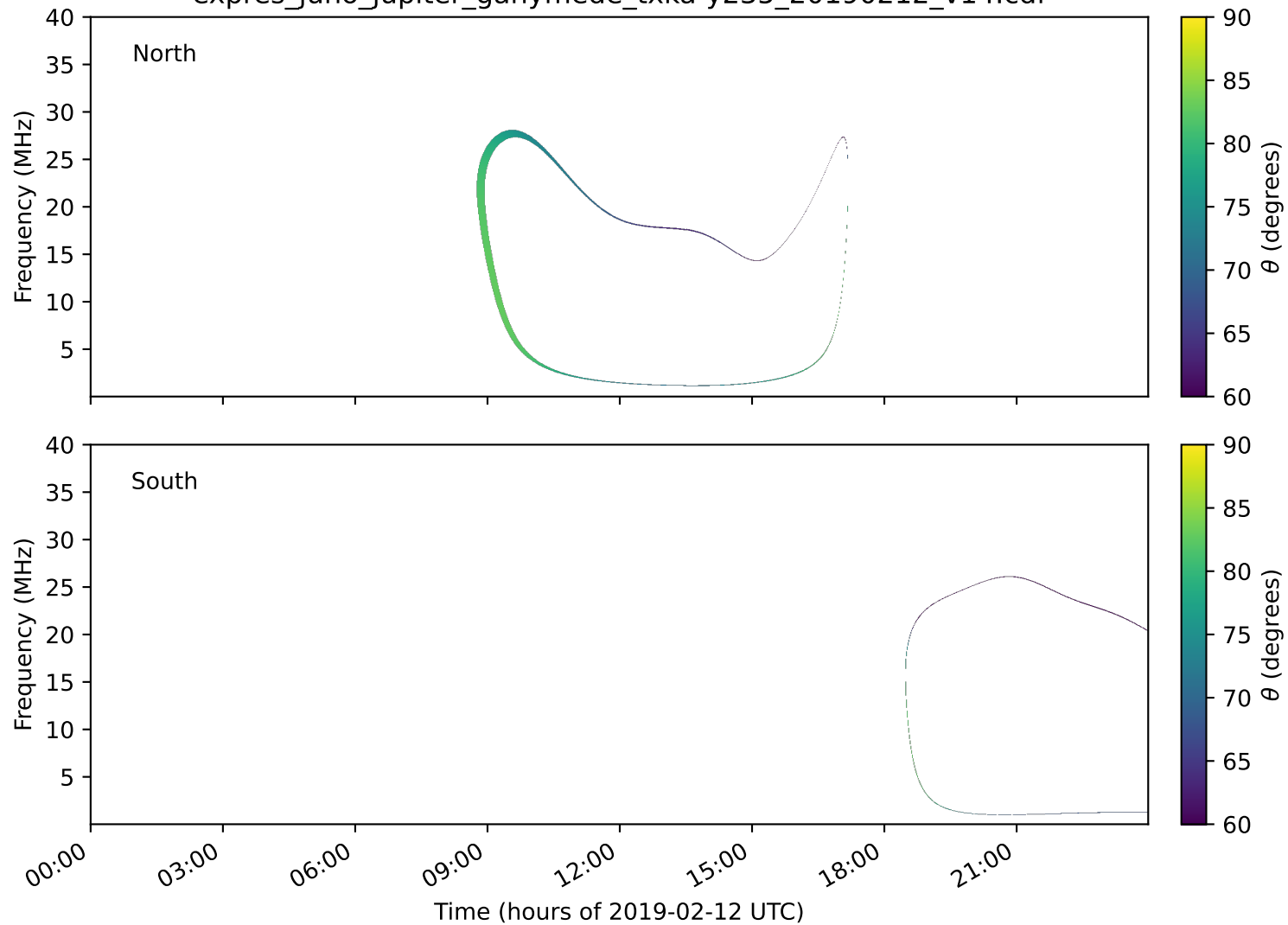
expres_juno_jupiter_ganymede_txka-y235_20190212_v14.cdf
