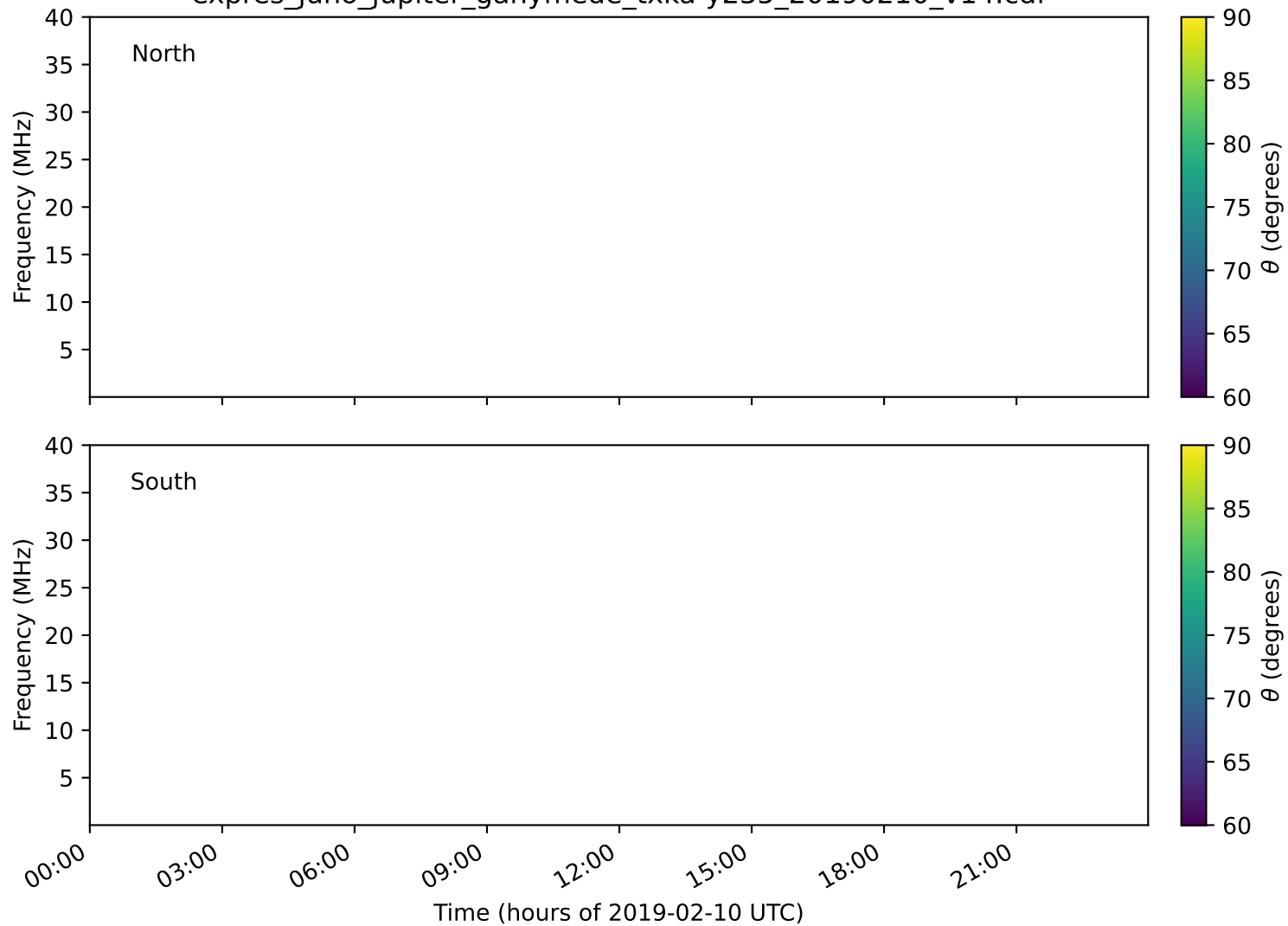
expres_juno_jupiter_ganymede_txka-y235_20190210_v14.cdf
