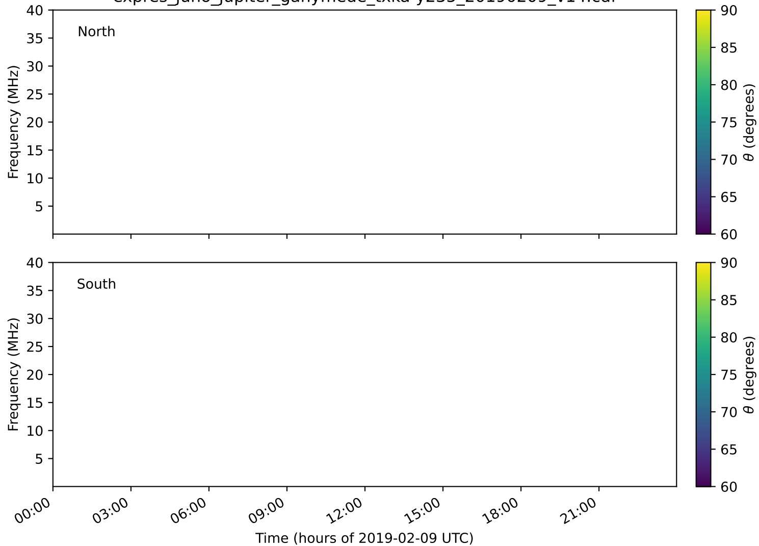
expres_juno_jupiter_ganymede_txka-y235_20190209_v14.cdf
