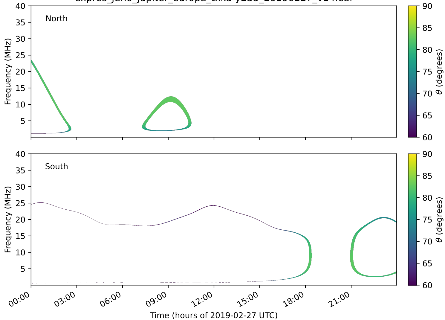
expres_juno_jupiter_europa_txka-y235_20190227_v14.cdf
