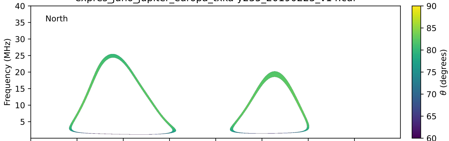
expres_juno_jupiter_europa_txka-y235_20190223_v14.cdf
