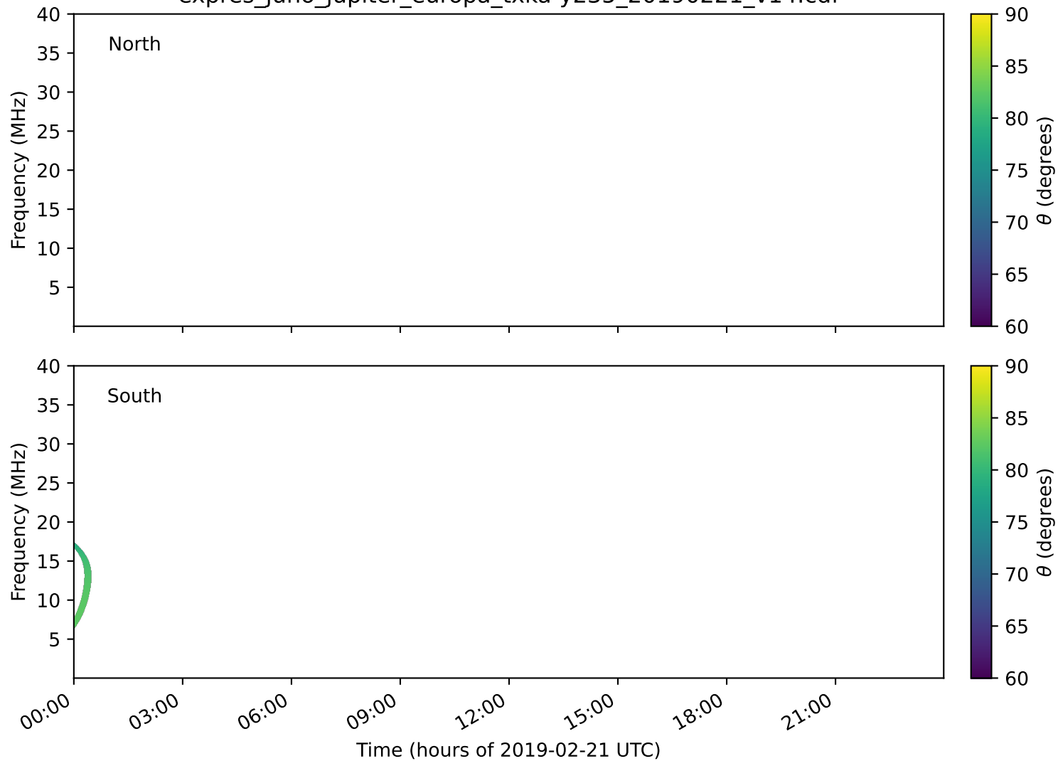
expres_juno_jupiter_europa_txka-y235_20190221_v14.cdf
