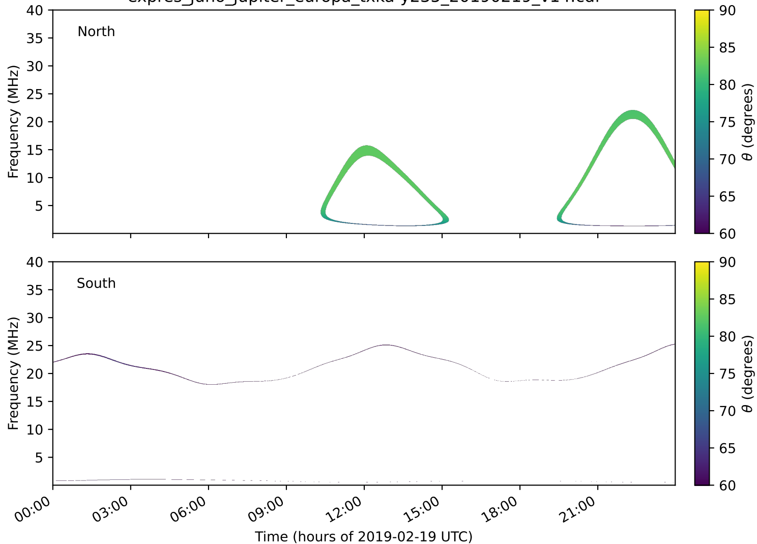
expres_juno_jupiter_europa_txka-y235_20190219_v14.cdf
