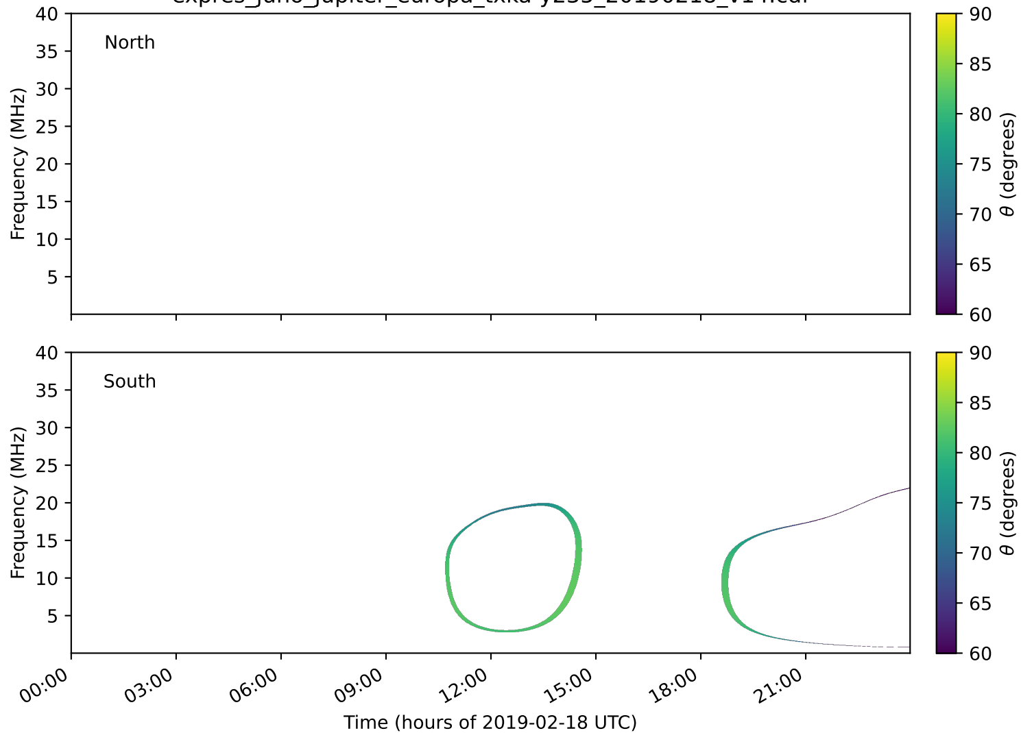
expres_juno_jupiter_europa_txka-y235_20190218_v14.cdf
