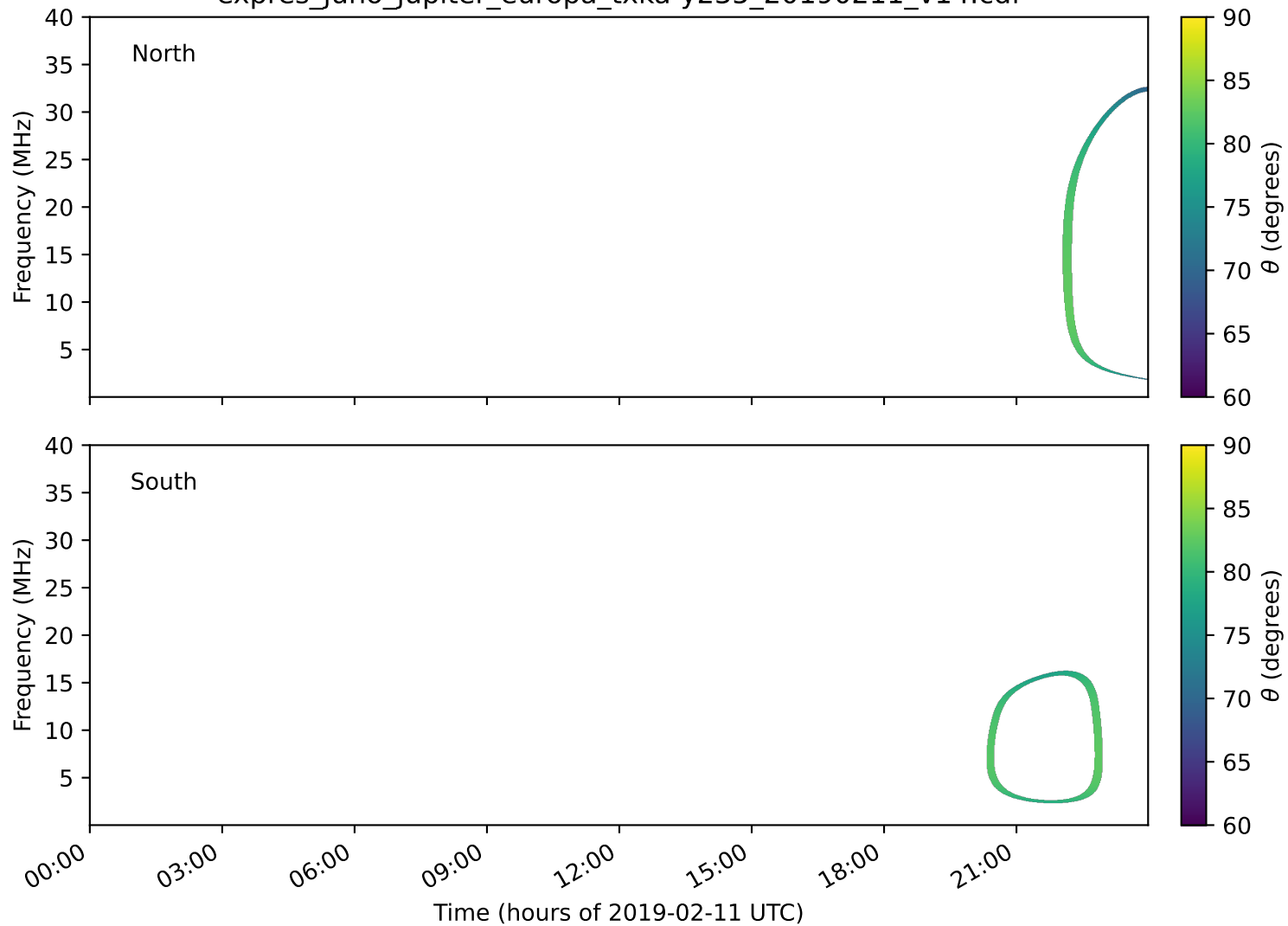
expres_juno_jupiter_europa_txka-y235_20190211_v14.cdf
