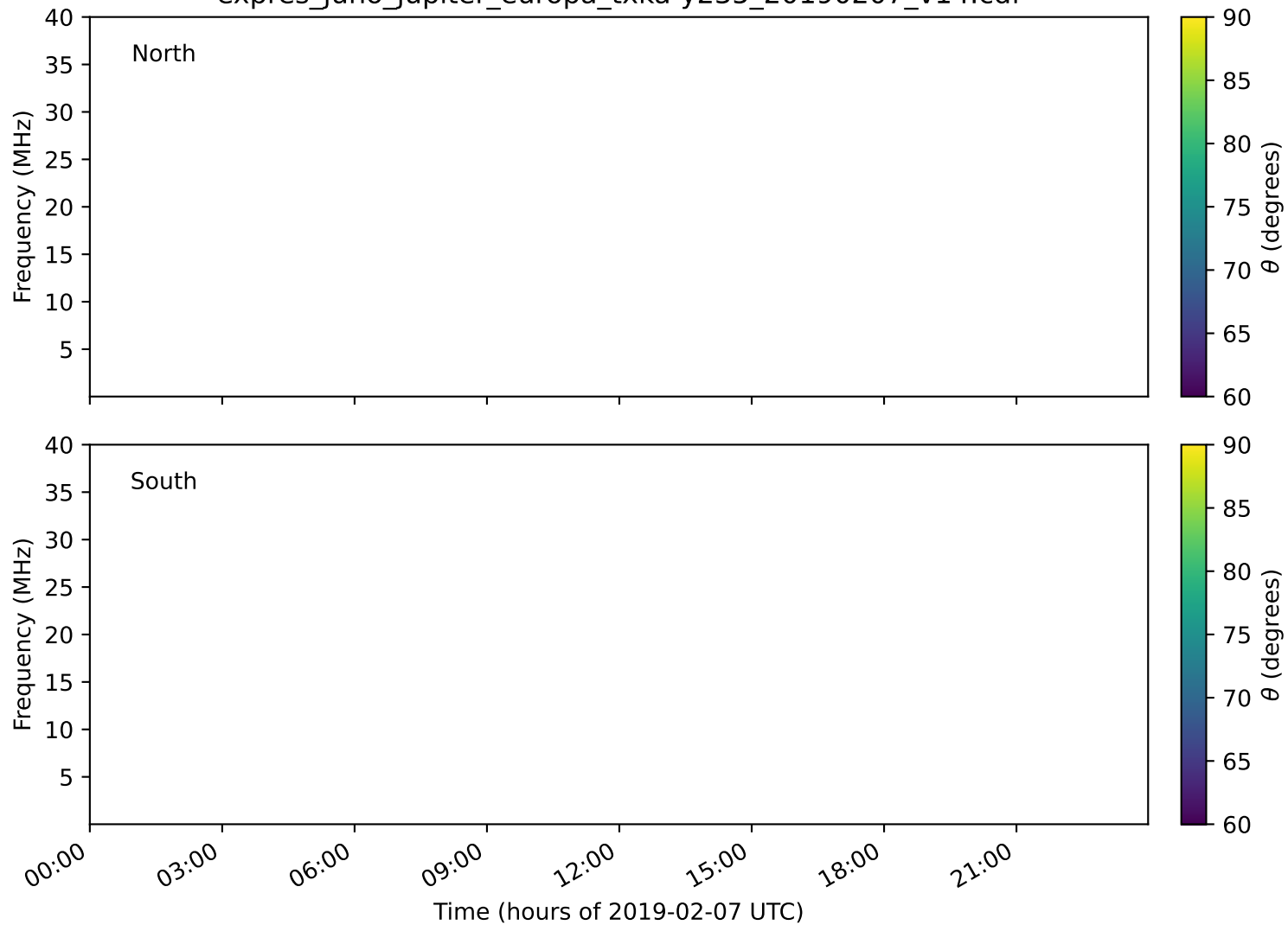
expres_juno_jupiter_europa_txka-y235_20190207_v14.cdf
