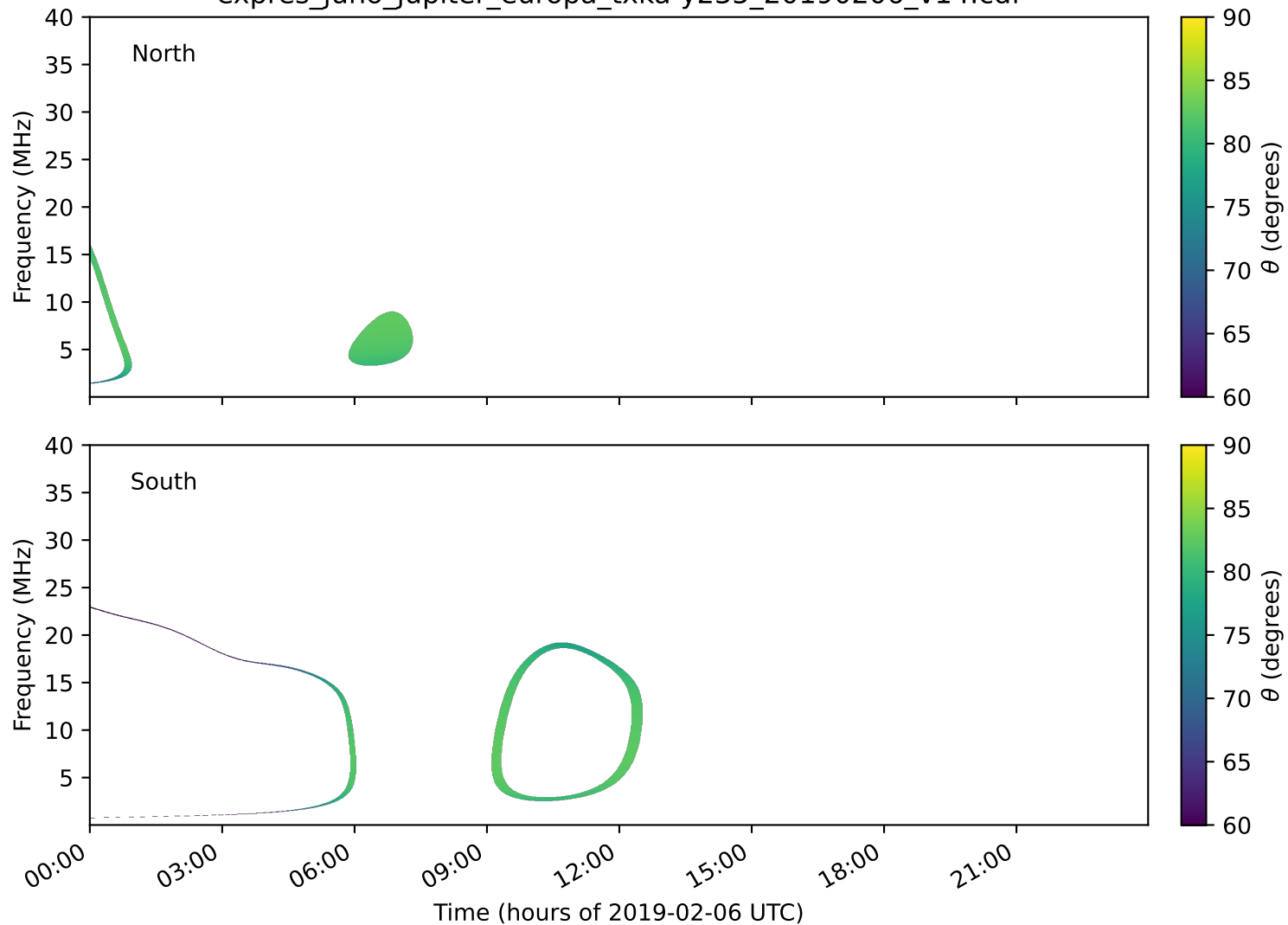
expres_juno_jupiter_europa_txka-y235_20190206_v14.cdf
