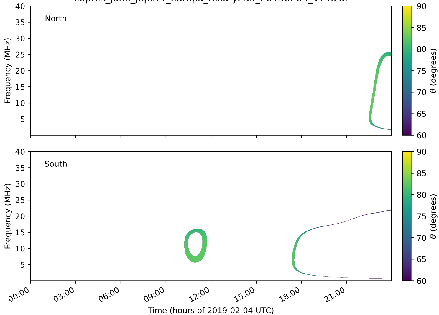
expres_juno_jupiter_europa_txka-y235_20190204_v14.cdf
