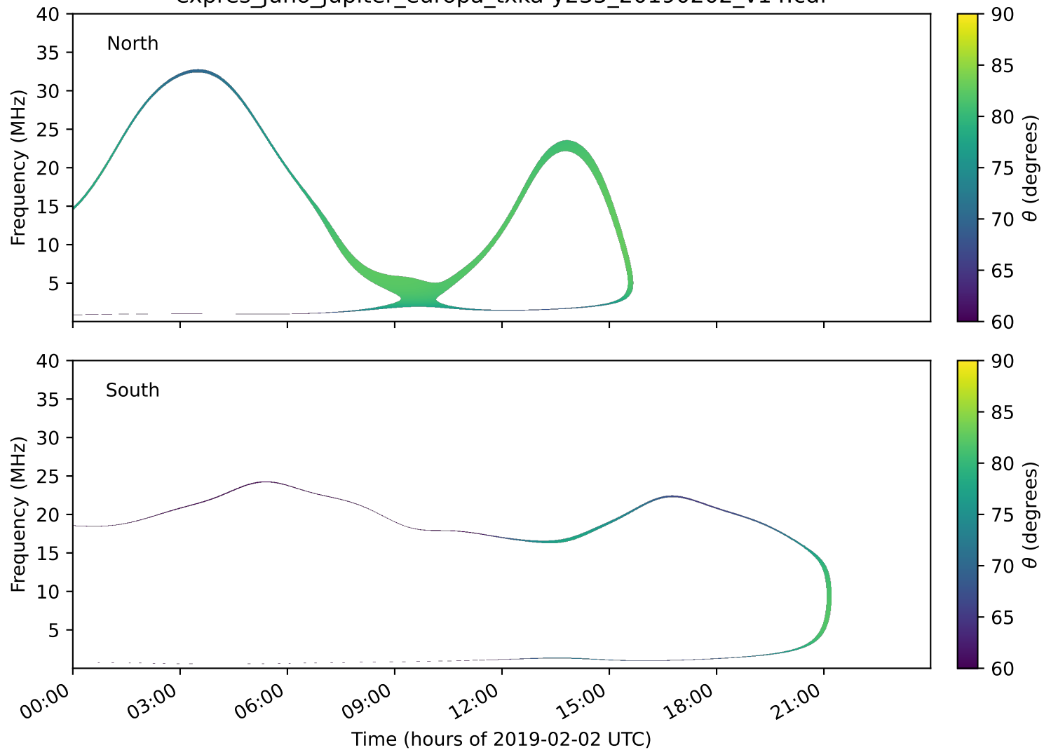
expres_juno_jupiter_europa_txka-y235_20190202_v14.cdf
