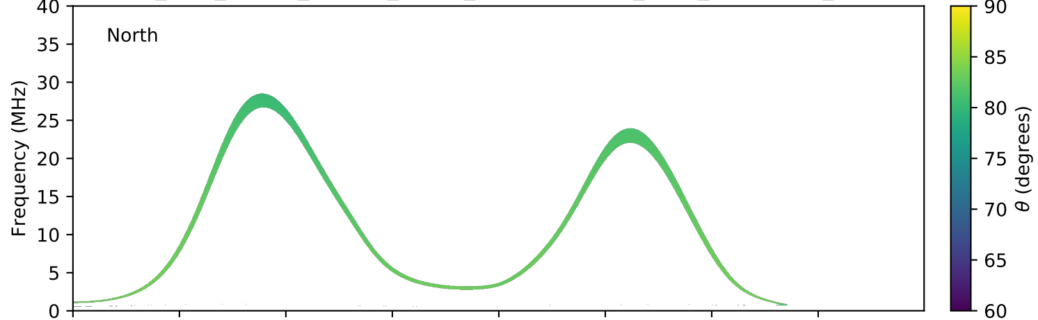
expres_juno_jupiter_europa_jrm09_lossc-wid1deg_3kev_20190223_v01.cdf
